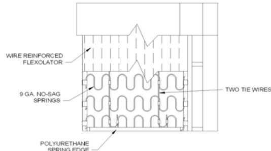
Seat Construction
